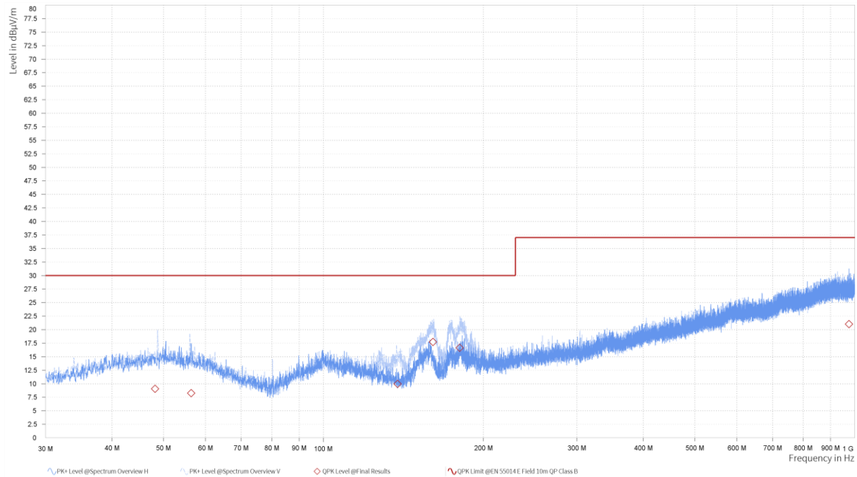
Radiated Emission 30M-1GHz
