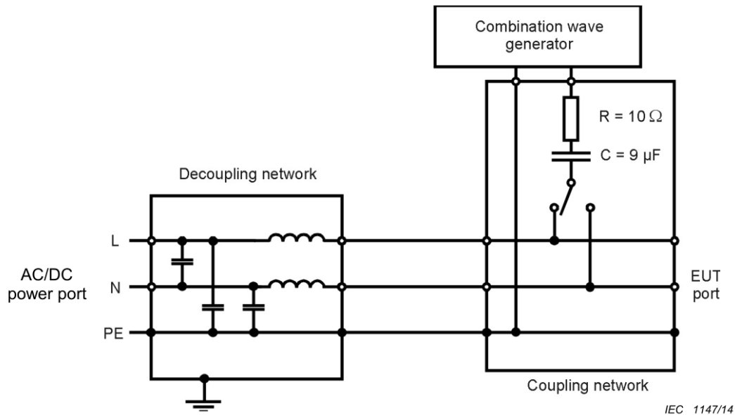
a.c./d.c. lines: line-to-ground coupling
