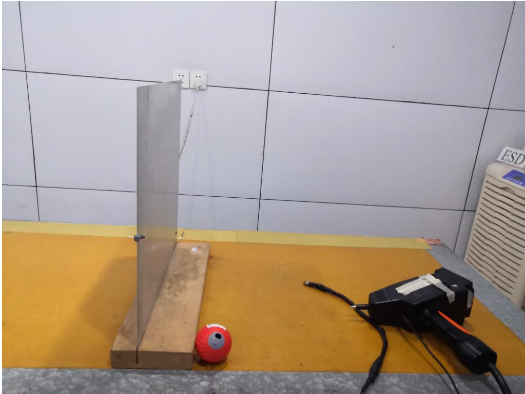
Picture 3 Electrostatic Discharge Test Setup
