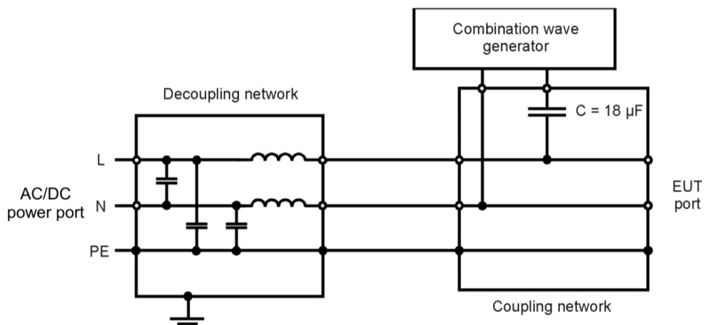
a.c./d.c. lines line-to-line coupling
